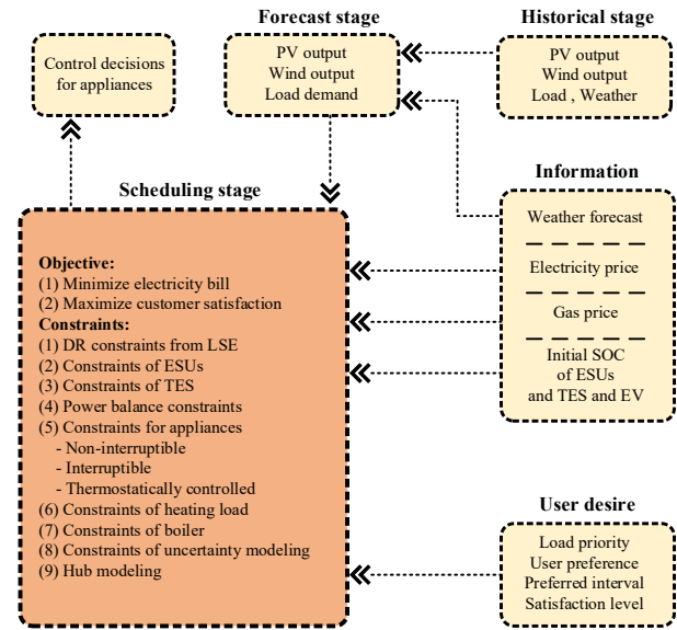
Fig. 2. The optimization framework of HEMS.
